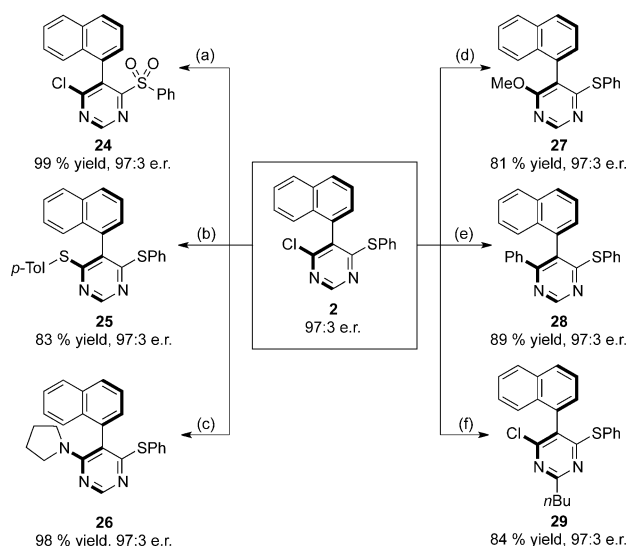
Scheme 3. Derivatization of substituted products. Reaction conditions: a) m CPBA (5.0 equiv), \text{CH}_2\text{Cl}_2 , RT, 16 h. b) p -thiocresol (1.3 equiv), 50% KOH (aq., w/w, 10 equiv), n\text{Bu}_4\text{NBr} (10 mol%), PhMe, RT, 16 h. c) pyrrolidine (5.0 equiv), \text{NEtPr}_2 (5.0 equiv), DMF, RT, 3 h. d) MeOH (5.0 equiv), \text{CsOH}\cdot\text{H}_2\text{O} (2.0 equiv), n\text{Bu}_4\text{NHSO}_4 (10 mol%), PhMe, RT, 24 h. e) \text{PhB(OH)}_2 (1.5 equiv), [\text{Pd}(\text{PPh}_3)_4] (10 mol%), \text{K}_2\text{CO}_3 (2.0 equiv), PhMe, 75^\circ\text{C} , 16 h. f) n\text{BuLi} (1.1 equiv), THF, -78^\circ\text{C} , 10 min, then \text{H}_2\text{O} , DDQ (1.1 equiv), -78^\circ\text{C} to RT, 5 min. DMF = N,N -dimethylformamide, m CPBA = m -chloroperbenzoic acid, THF = tetrahydrofuran.
